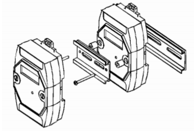
Fig.3 DAM-E3043 stack installation
